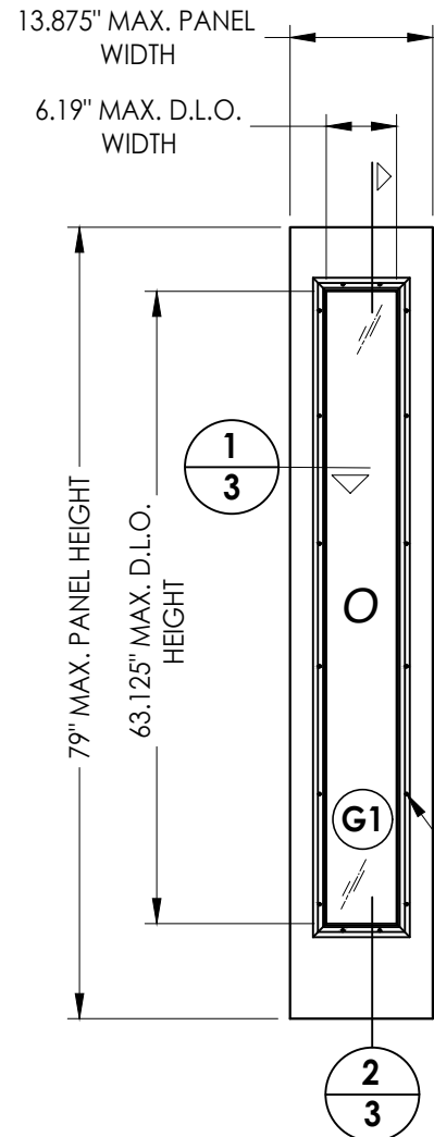
50 FIBERGLASS SIDELITE PANEL ODL LITE FRAME (HP POLY PRO)
