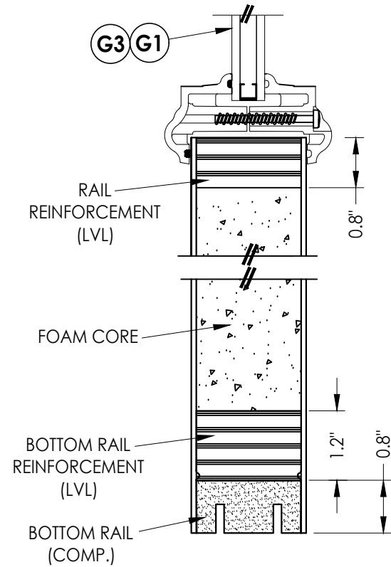
2 VERTICAL CROSS SECTION
