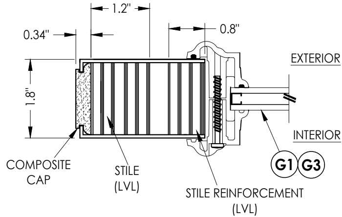
1 HORIZONTAL CROSS SECTION 3
